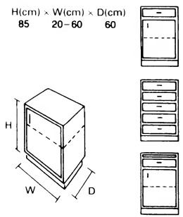
① Single floor unit
